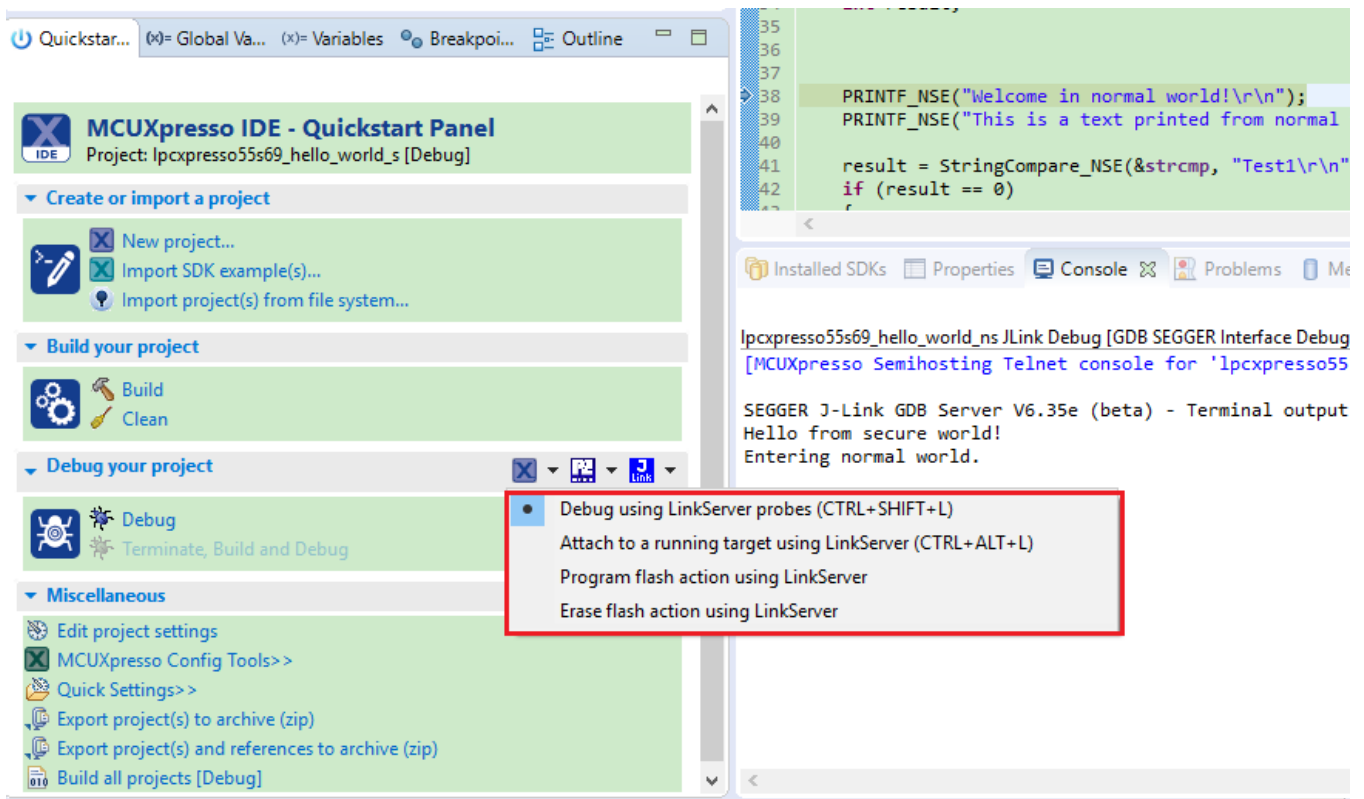
Figure 36. Debug lpcxpresso55s69_hello_world_s case
