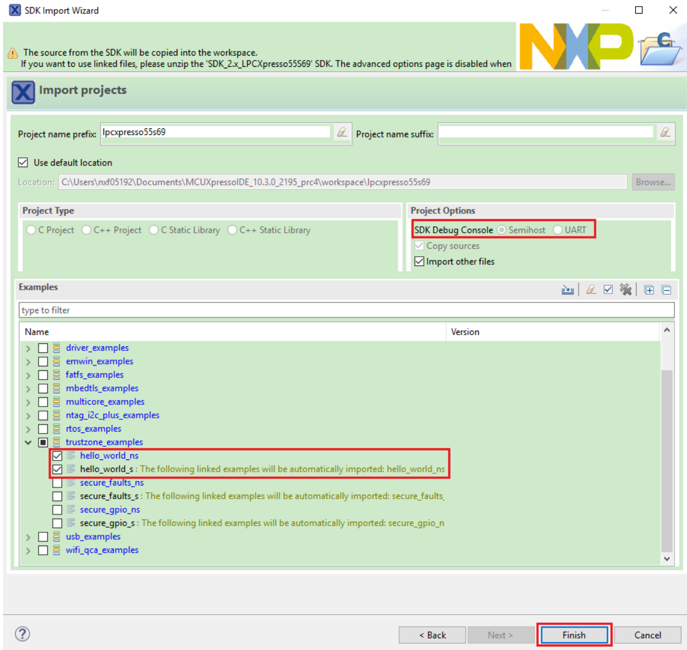
Figure 29. Select the hello_world TrustZone example
