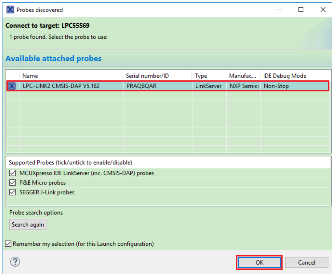
Figure 33. Attached Probes: debug emulator selection
