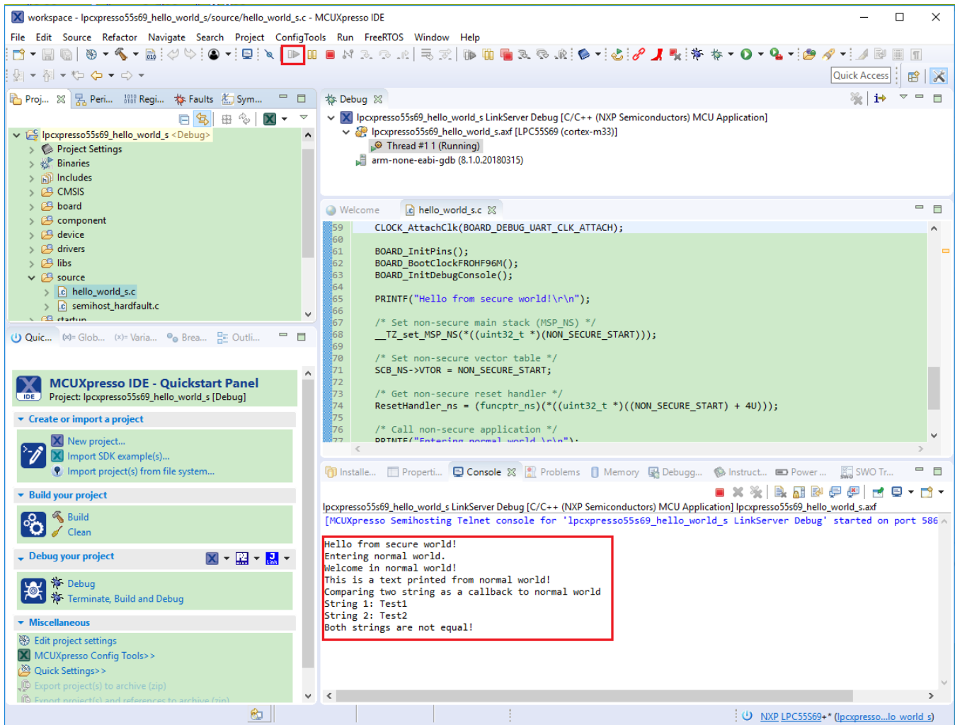
Figure 38. Run Hello World trustzone example and get the message
