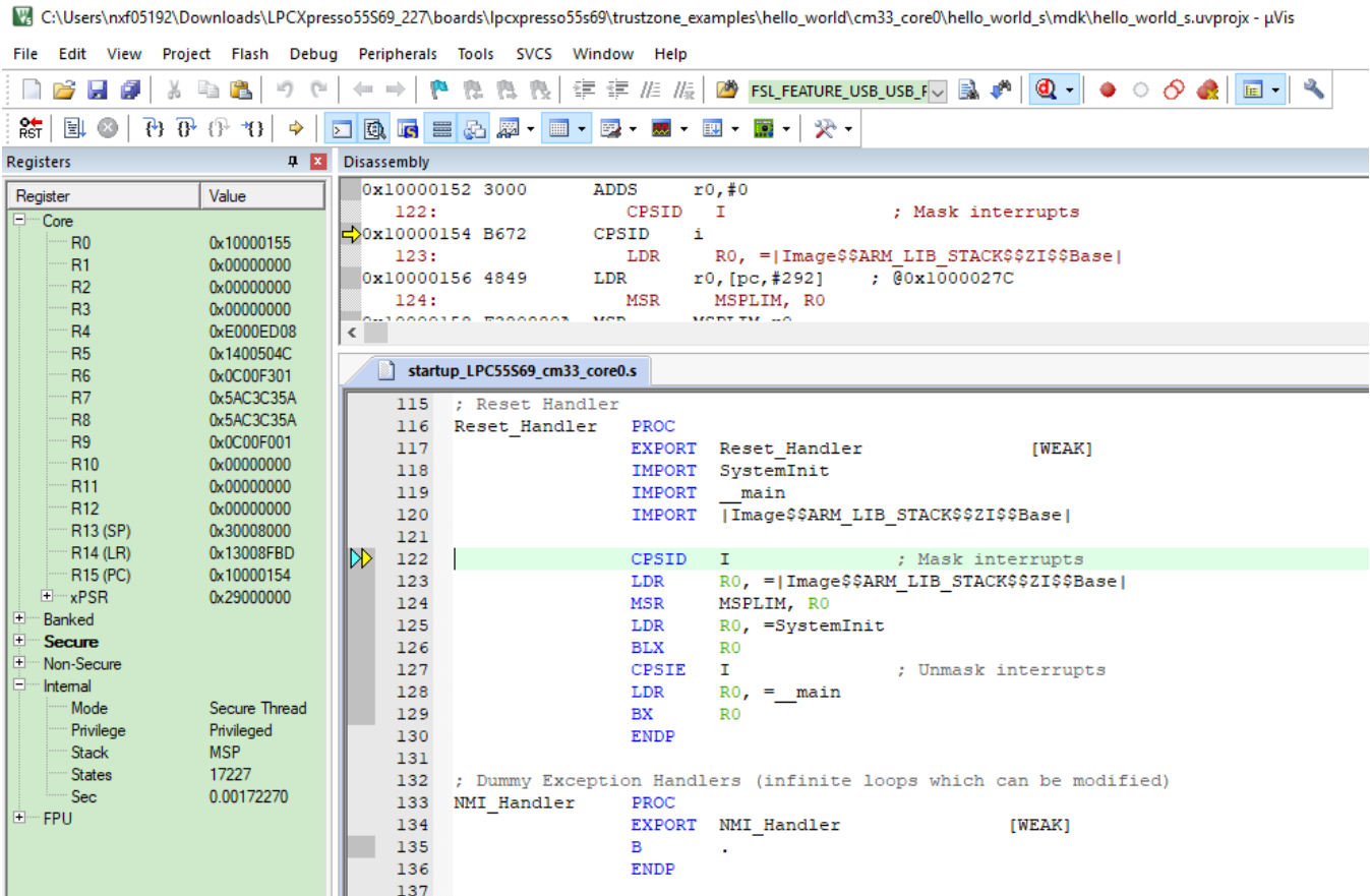
Figure 60. Stop at Rest_Handler when running debugging
