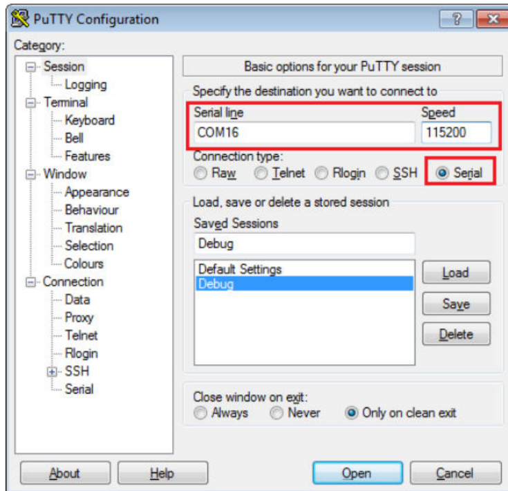
Figure 54. Terminal (PuTTY) configurations
