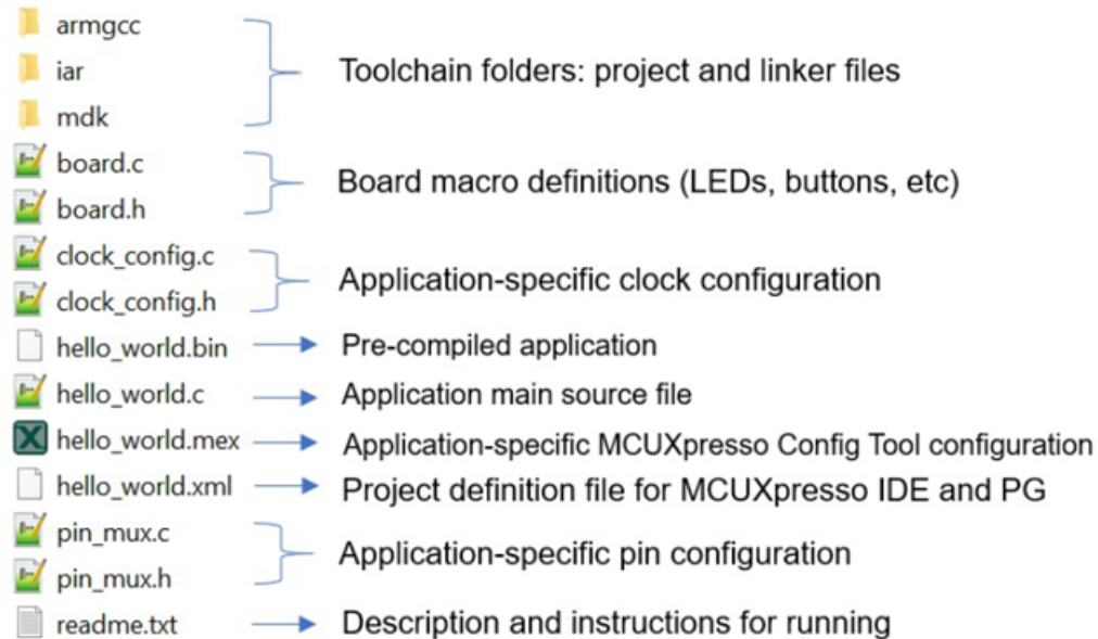
Figure 2. Application folder structure
