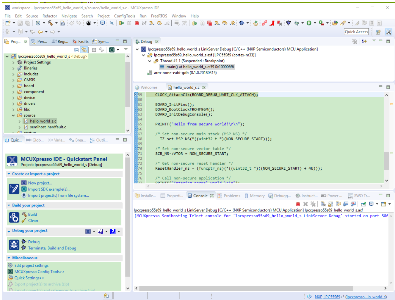
Figure 37. Debug the hello_world_s project
