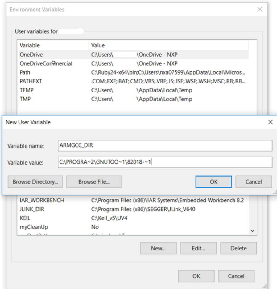
Figure 67. Add ARMGCC_DIR system variable
