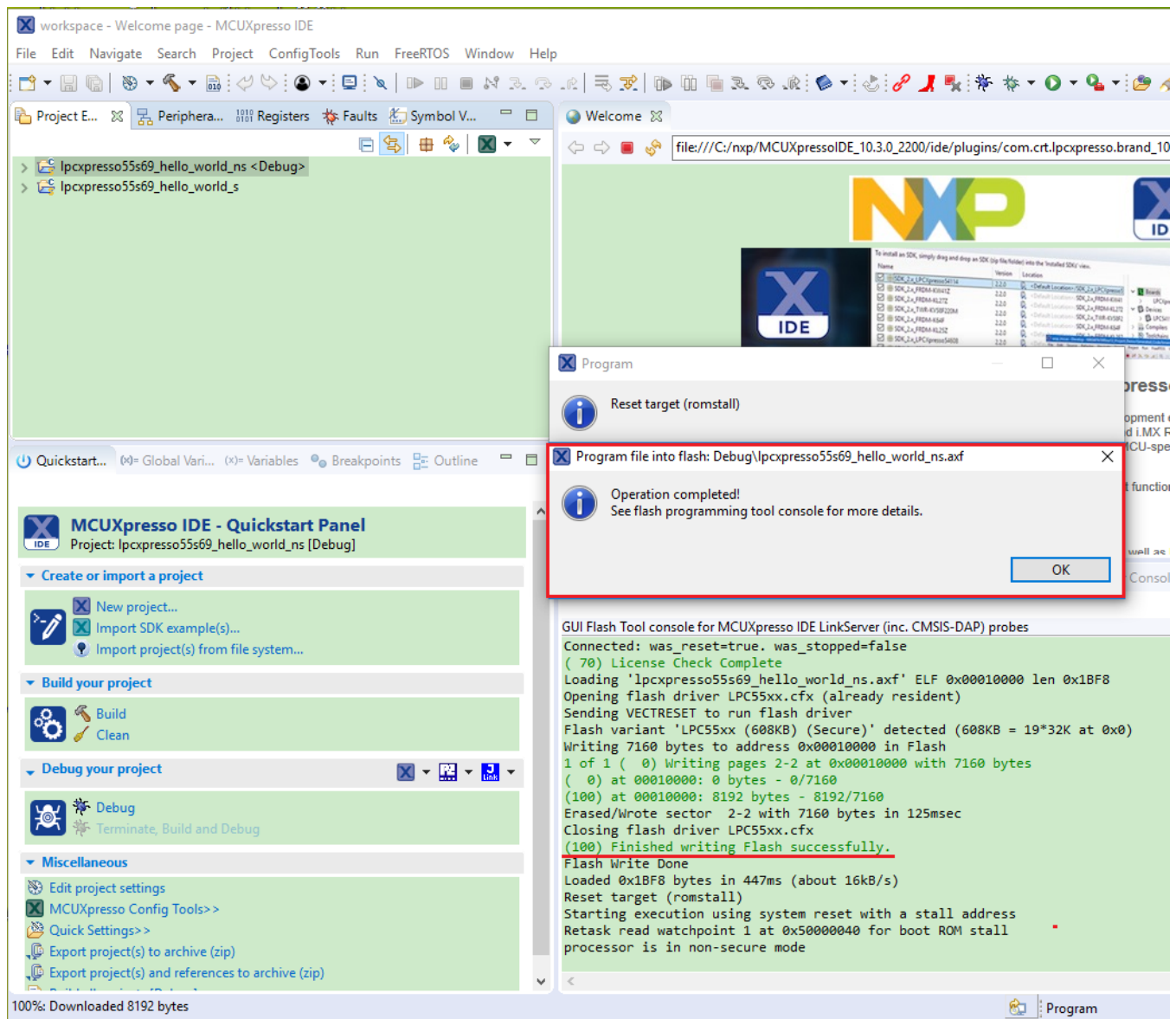
Figure 35. Load lpcpresso55s69_hello_world_ns.axf
