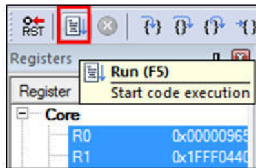
Figure 61. Go button
