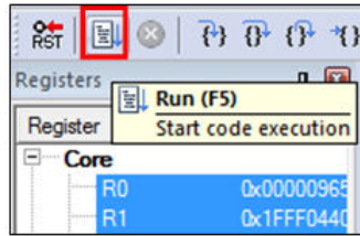
Figure 56. Go button
