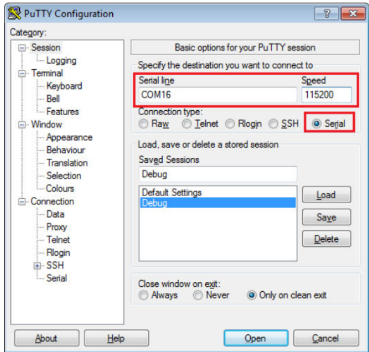
Figure 71. Terminal (PuTTY) configurations
