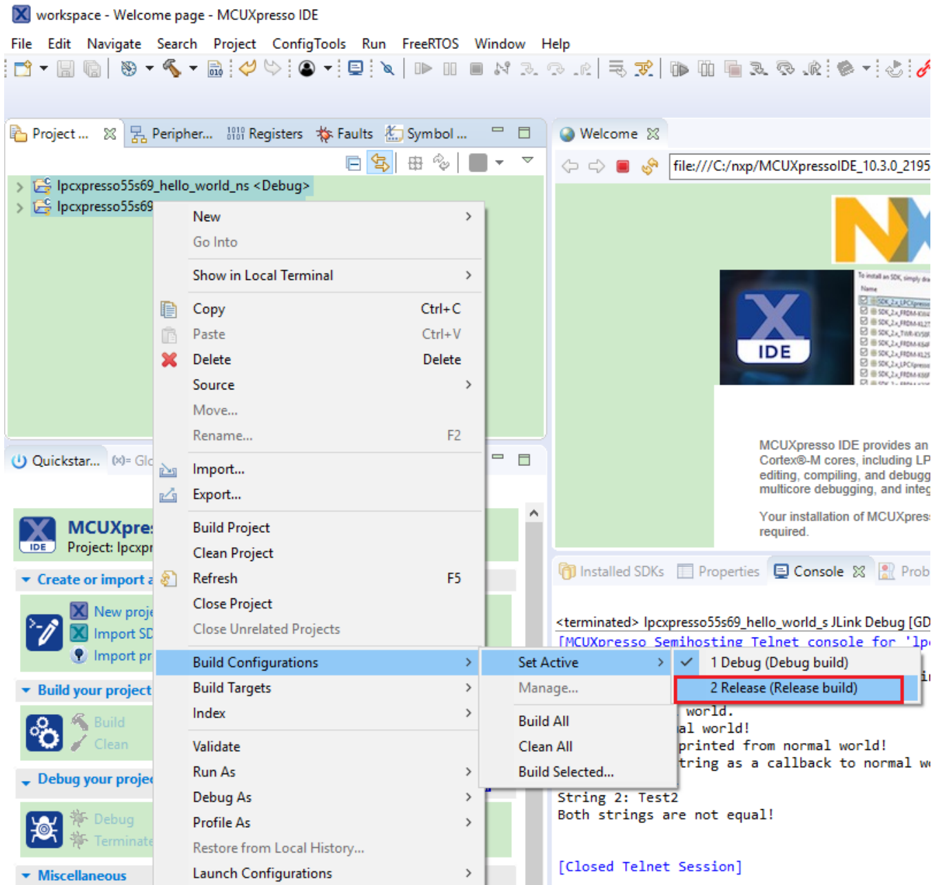
Figure 31. Switching TrustZone projects into the Release build configuration
