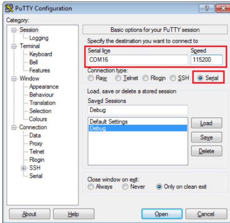
Figure 41. Terminal (PuTTY) configuration
