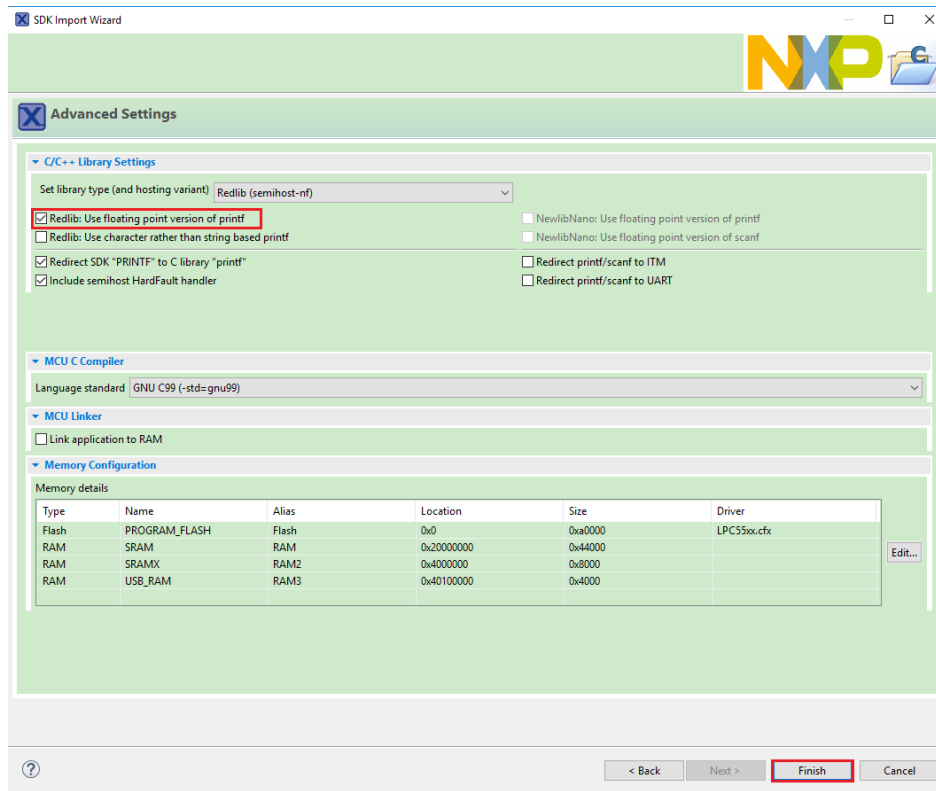
Figure 7. Select Use floating point version of printf
