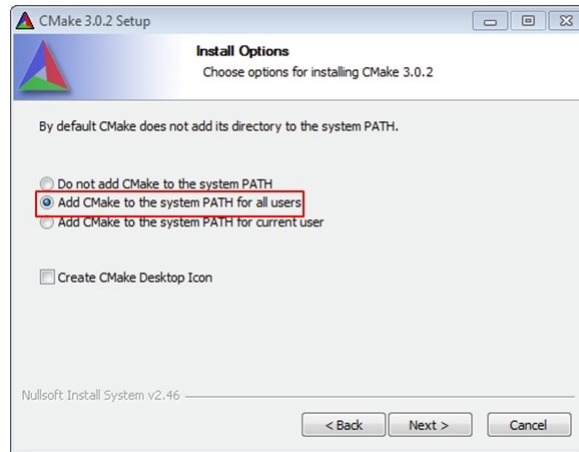
Figure 68. Install CMake
