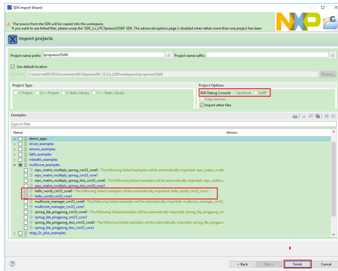
Figure 15. Select the hello_world multicore example
