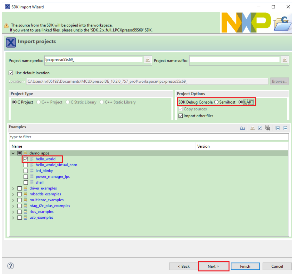
Figure 6. Select hello_world
