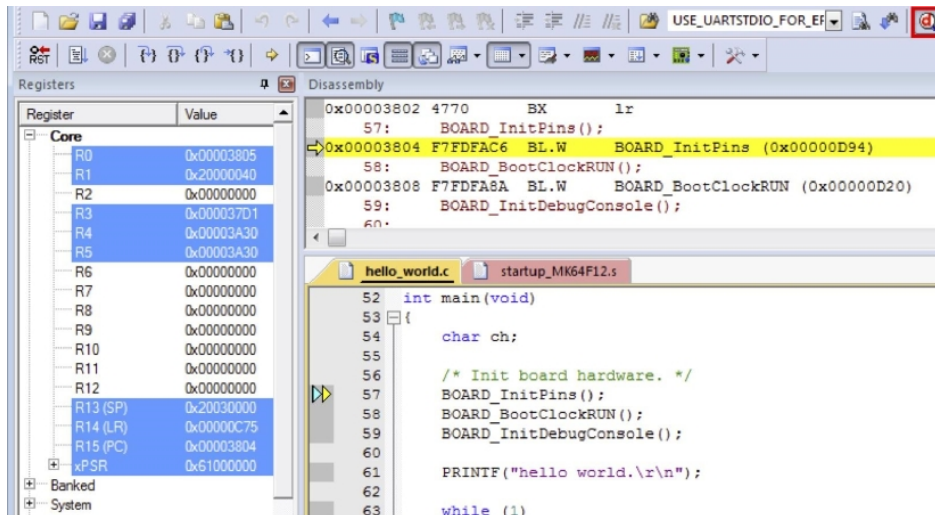
Figure 55. Stop at main() when run debugging
