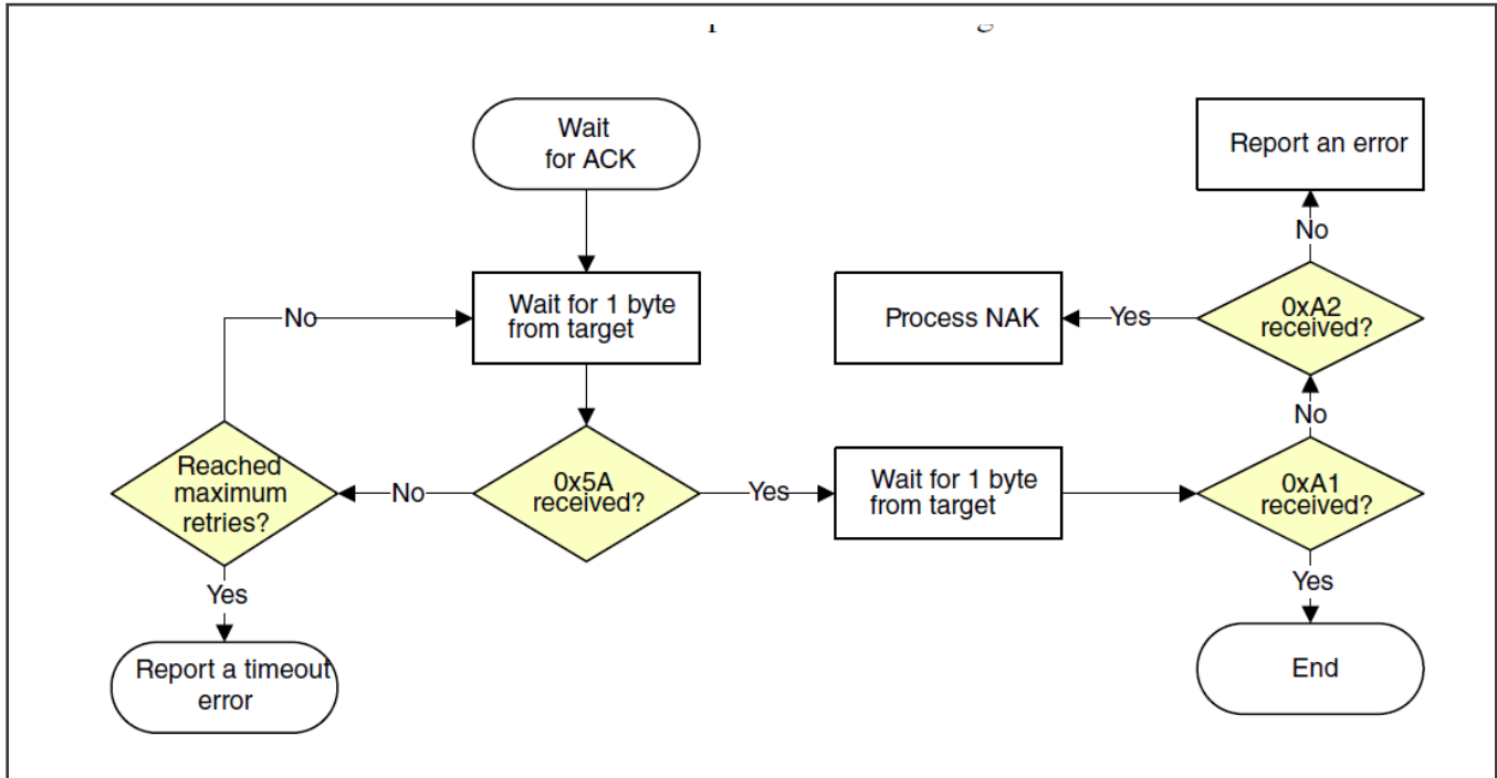
Figure 18. Host reads an ACK from target via UART
