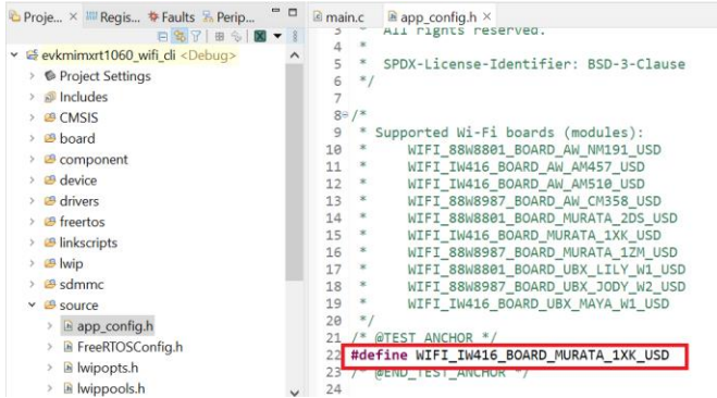
Figure 5: Wi-Fi Module Selection in MCUXpresso
