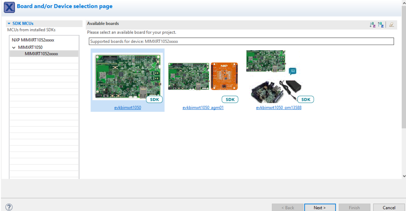
Figure 27. Selecting EVKB-IMXRT1050 board
