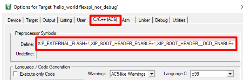
Figure 36. Options for target
