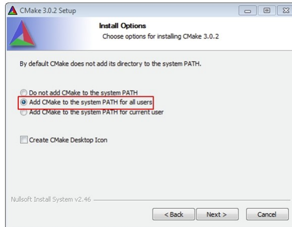
Figure 18. Install CMake
