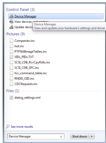
Figure 34. Device Manager
