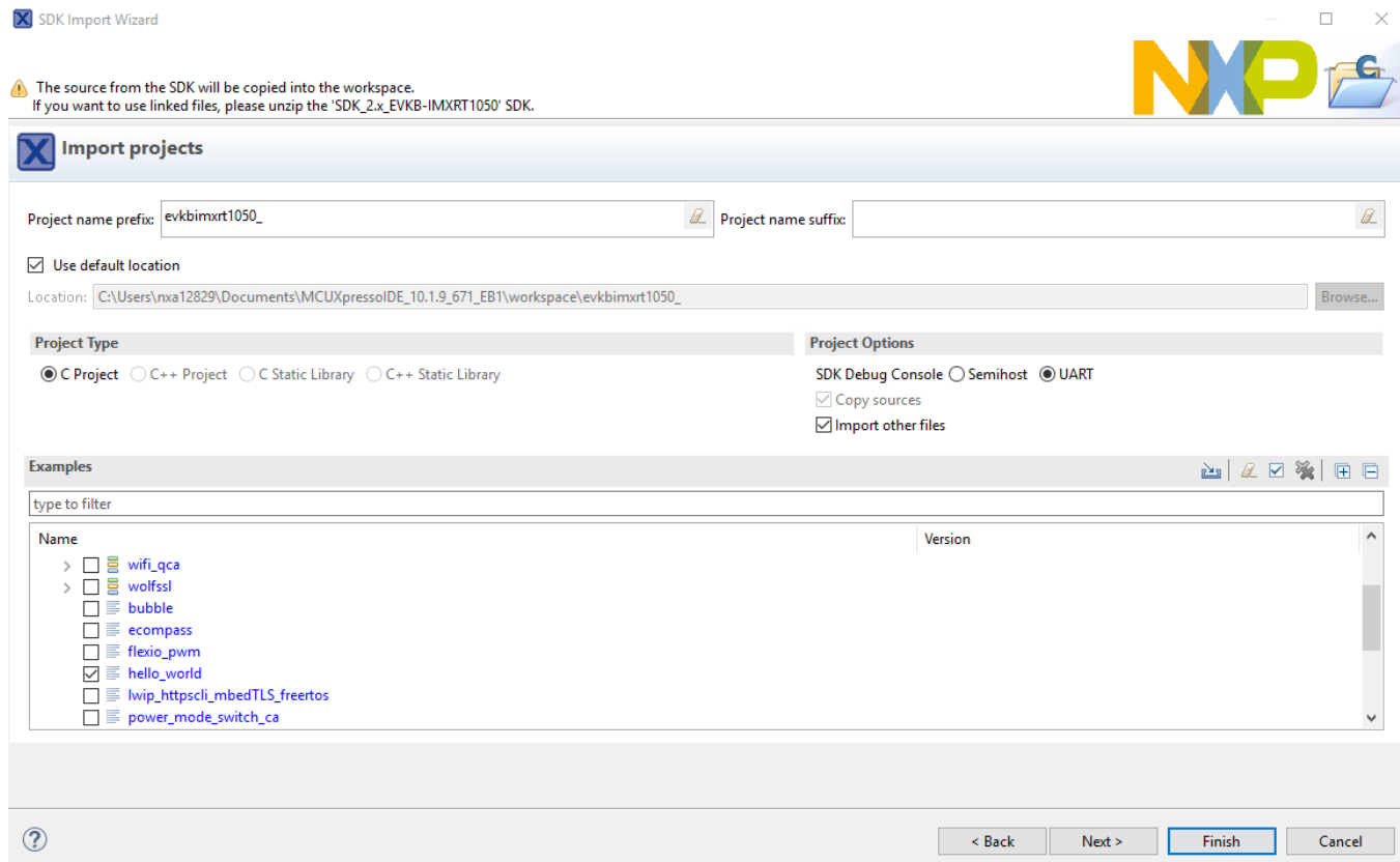
Figure 28. Selecting hello_world
