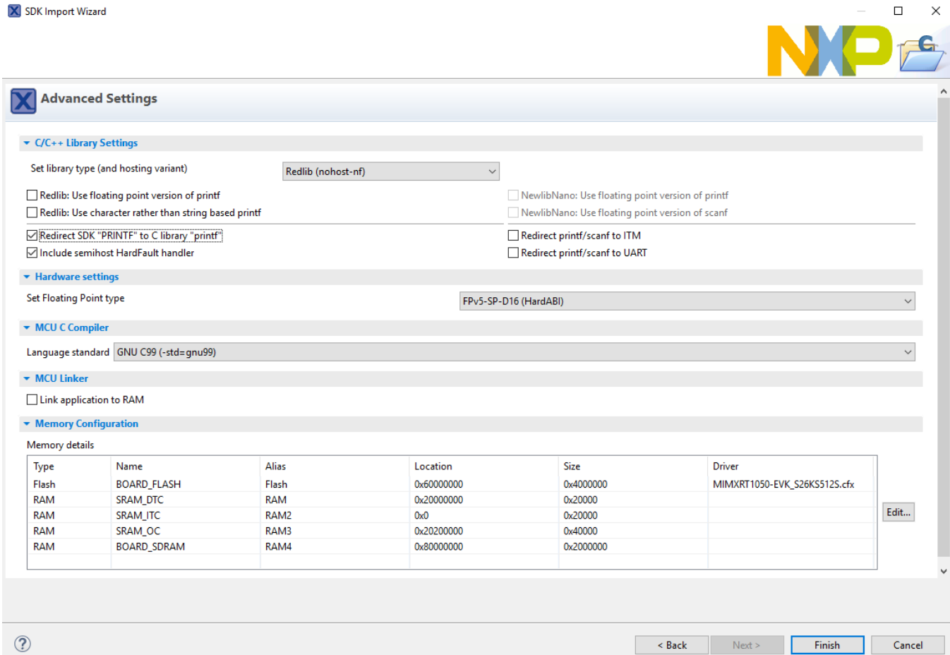
Figure 29. Selecting User floating point version of printf
